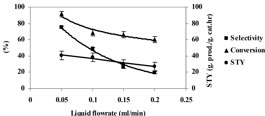
Figure 5. Effect of liquid flowrate on reactor performance
