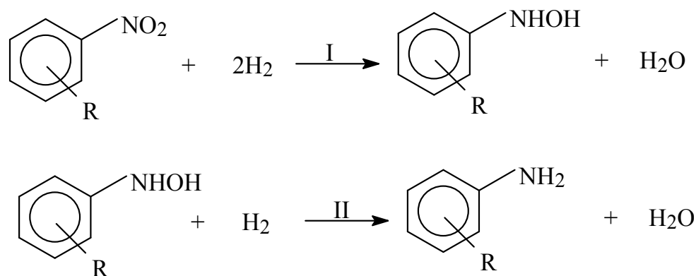
Figure 16. Reaction pathway for the hydrogenation of nitro compound
